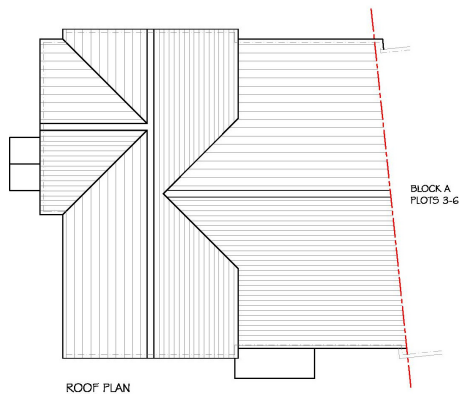
ROOF PLAN PLOTS 1-2
