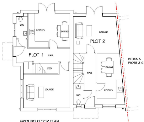
GROUND FLOOR PLAN PLOTS 1-2
